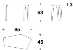
CTD (20) SIDE TABLE 85x45x53H.cm
