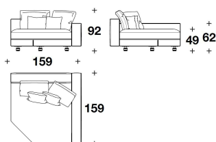
AZA (CLD) - AZA (CLS) CHAISE LONGUE DX O SX / RIGHT OR LEFT CHAISE LONGUE 159x159x92H. - H.A.62 - H.S.49 cm 62 2/3x62 2/3x36 1/3H. - H.A.24 1/3 - H.S.19 1/4 "
