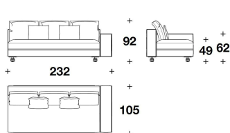
AZA (E3D) - AZA (E3S) ELEMENTO 3 POSTI CON BRACCIOLO DX O SX / 3 SEATER ELEMENT WITH RIGHT OR LEFT ARMREST 232x105x92H. - H.A.62 - H.S.49 cm 91 1/3x41 1/3x36 1/3H. - H.A.24 1/3 - H.S.19 1/4 "
