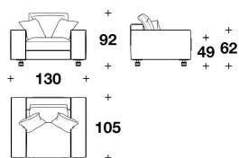
AZA (POL) POLTRONA / ARMCHAIR 130x105x92H. - H.A.62 - H.S.49 cm 51 1/3x41 1/3x36 1/3H. - H.A.24 1/3 - H.S.19 1/4 "
