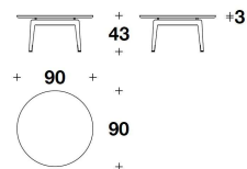
CTD (03) ROUND : COFFEE TABLE Ø 90x43H.cm
