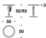
CTD (18) SIDE TABLE Ø 50x52-62H.cm Ø 19 3/4x20 1/3-24 1/3H."
