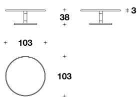
CTD (25) COFFEE TABLE 103x103x38H. - THK.3cm 40 2/3x40 2/3x15H. - THK.1 3/16"
